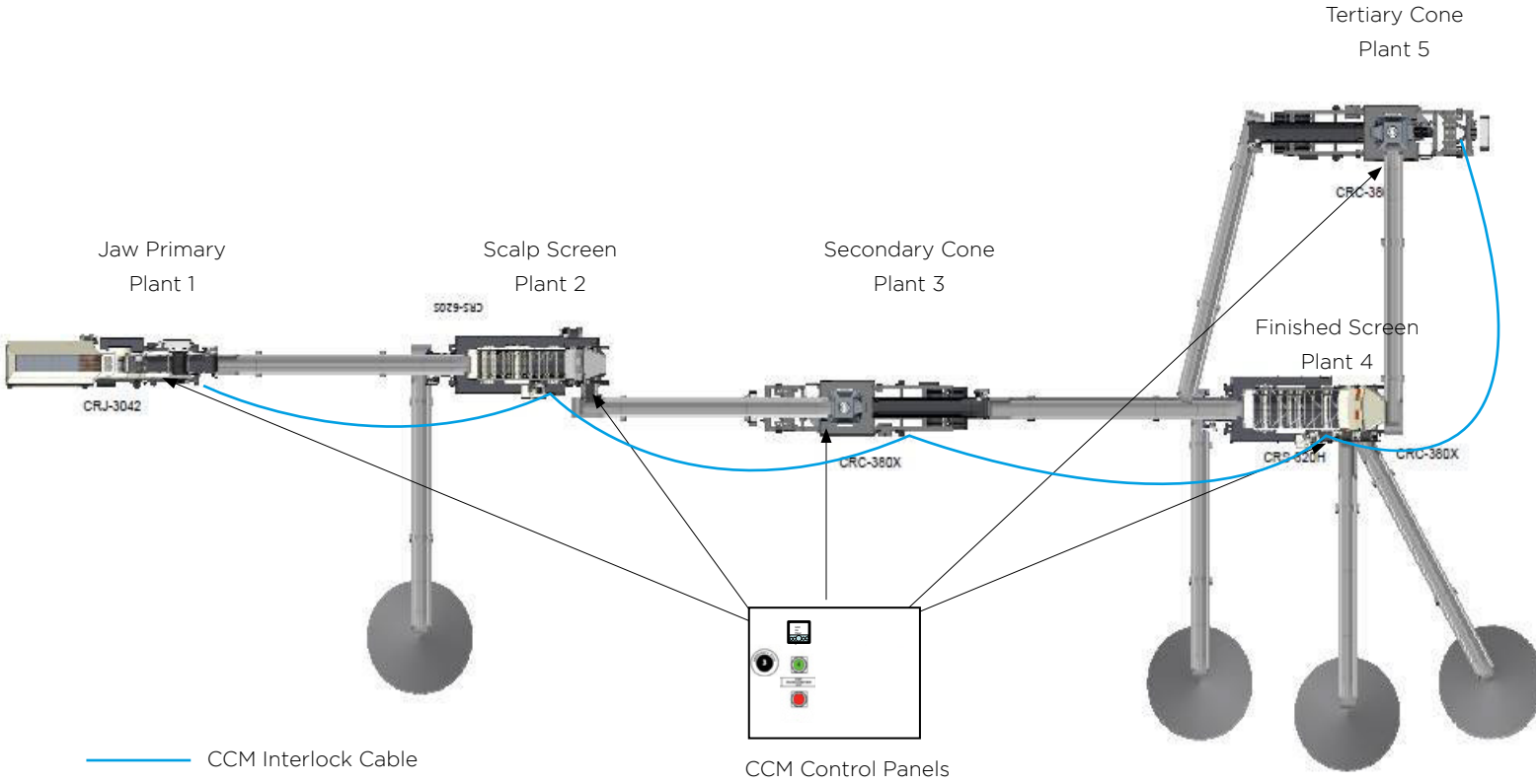
Diagram Showing CCM Control Panels and Interlock Cable
